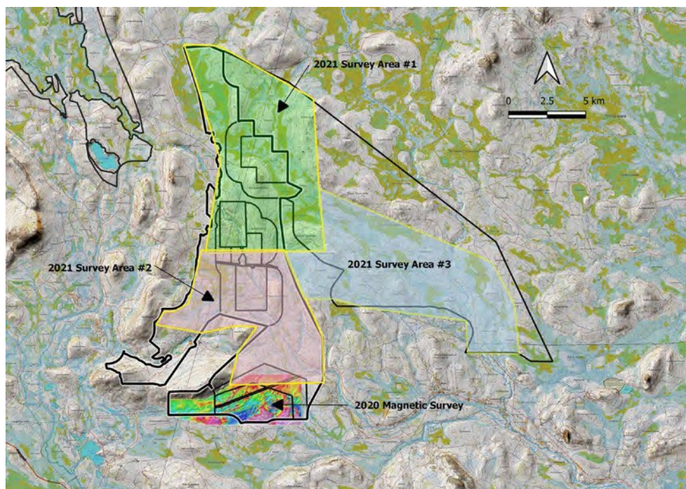
Figure 16. UAV Magnetic Survey Areas at the Northern Group Gold Properties to Q1 2022
