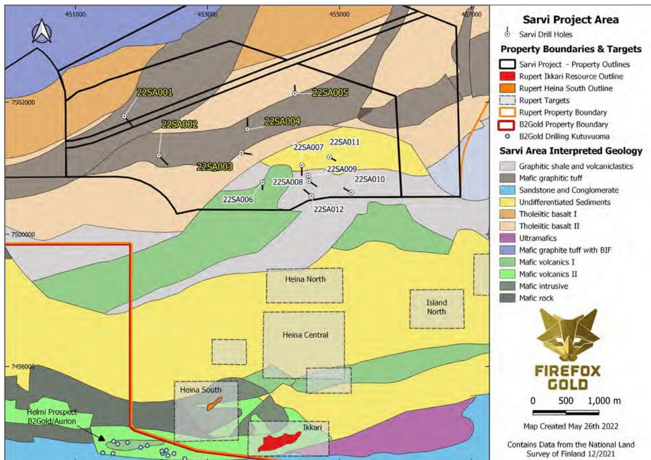
Figure 15. Initial reconnaissance drilling and interpreted geology at the Sarvi Project.
