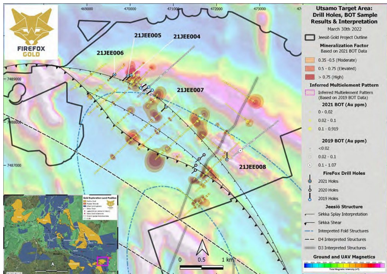
Figure 4. BOT Survey and Structure in Utsamo Corridor at Jeessio Project
