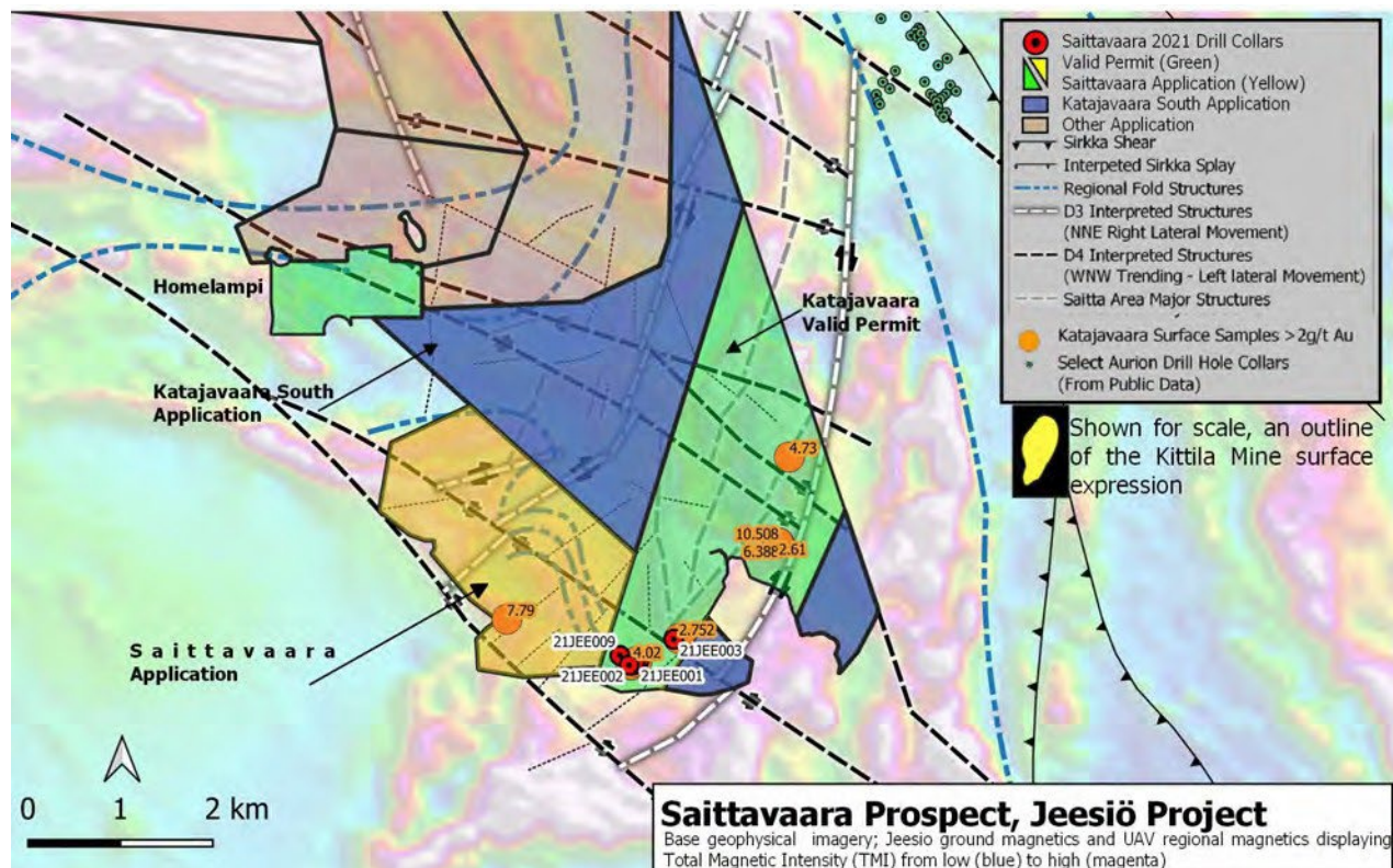
Figure 5. Saittavaara Prospect drill hole locations presented with FireFox's structural interpretation for the Jeesiö Project
