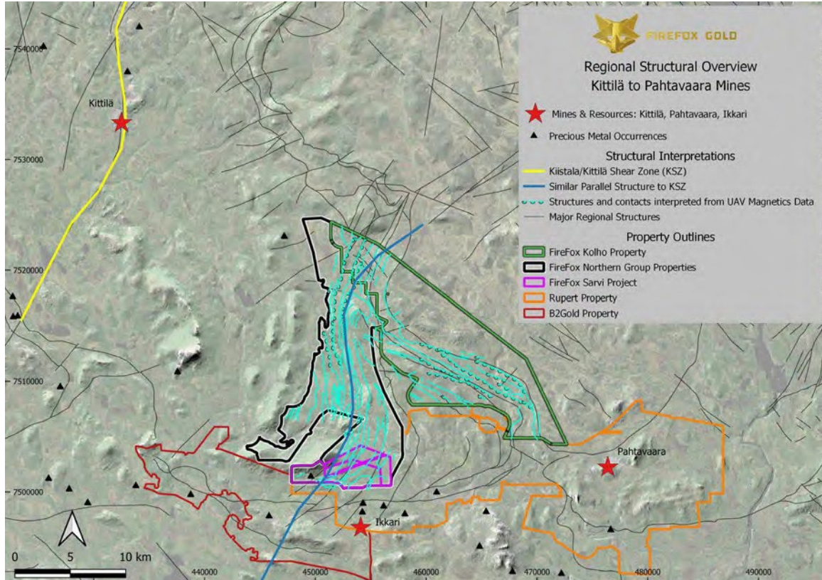
Figure 18. Regional structural overview through Northern Properties.
