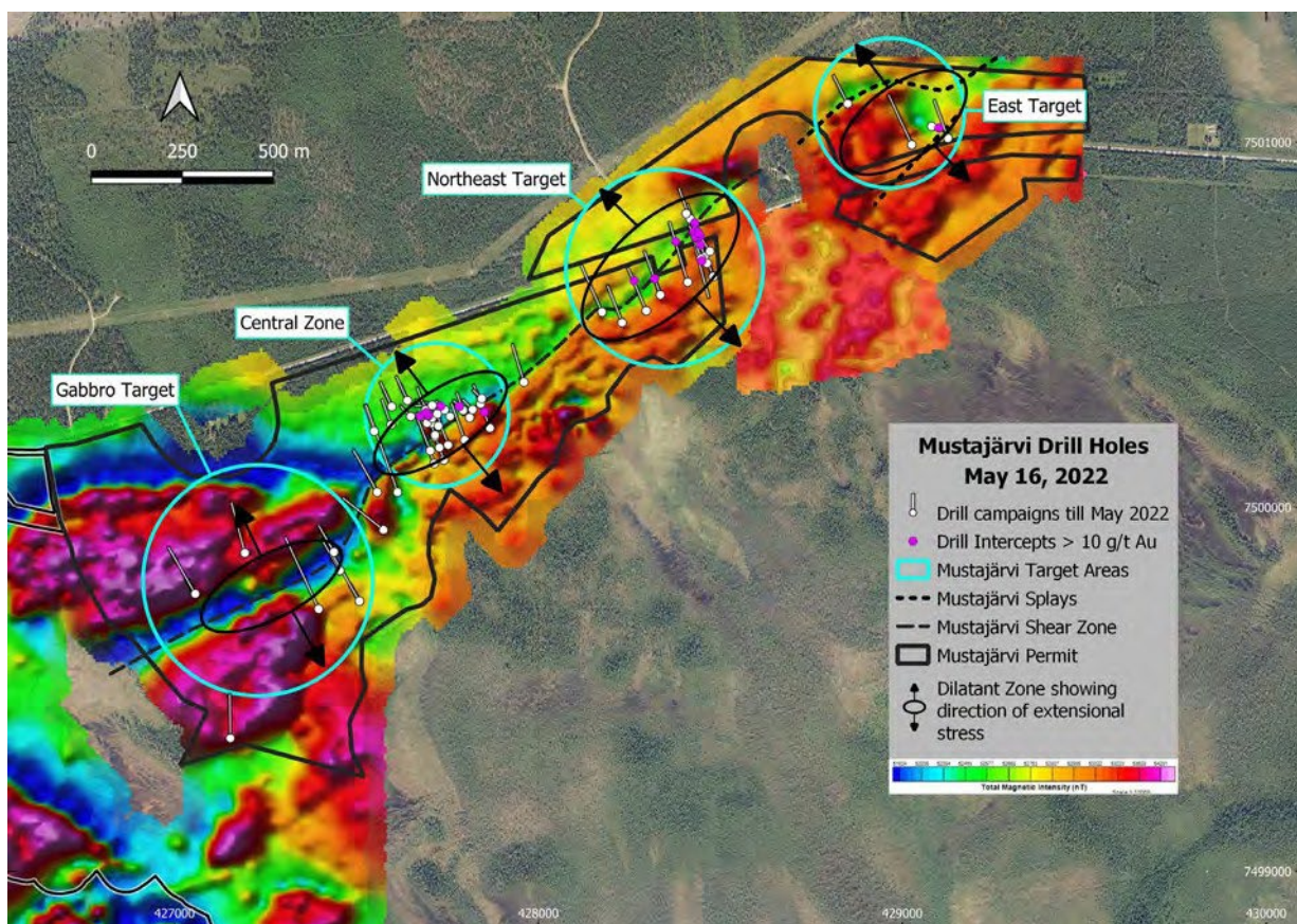
Figure 13. Mustajärvi Drill Collar Locations Relative to Structural Interpretation over Magnetics, May 16, 2022
